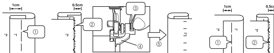
① :Basting ② :Sewing position ③ :Turn screw to adjust guide to folded hem. ④ :Guide ⑤ :Turn to front side *1 :Front side *2 :Reverse side
