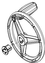
Hand-wheel Assy w/insert (1) QF09318-09325
